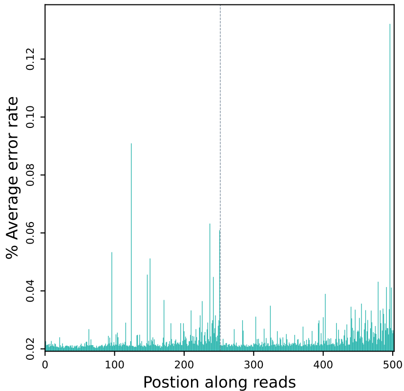
Error rate distribution along reads (R10210)
